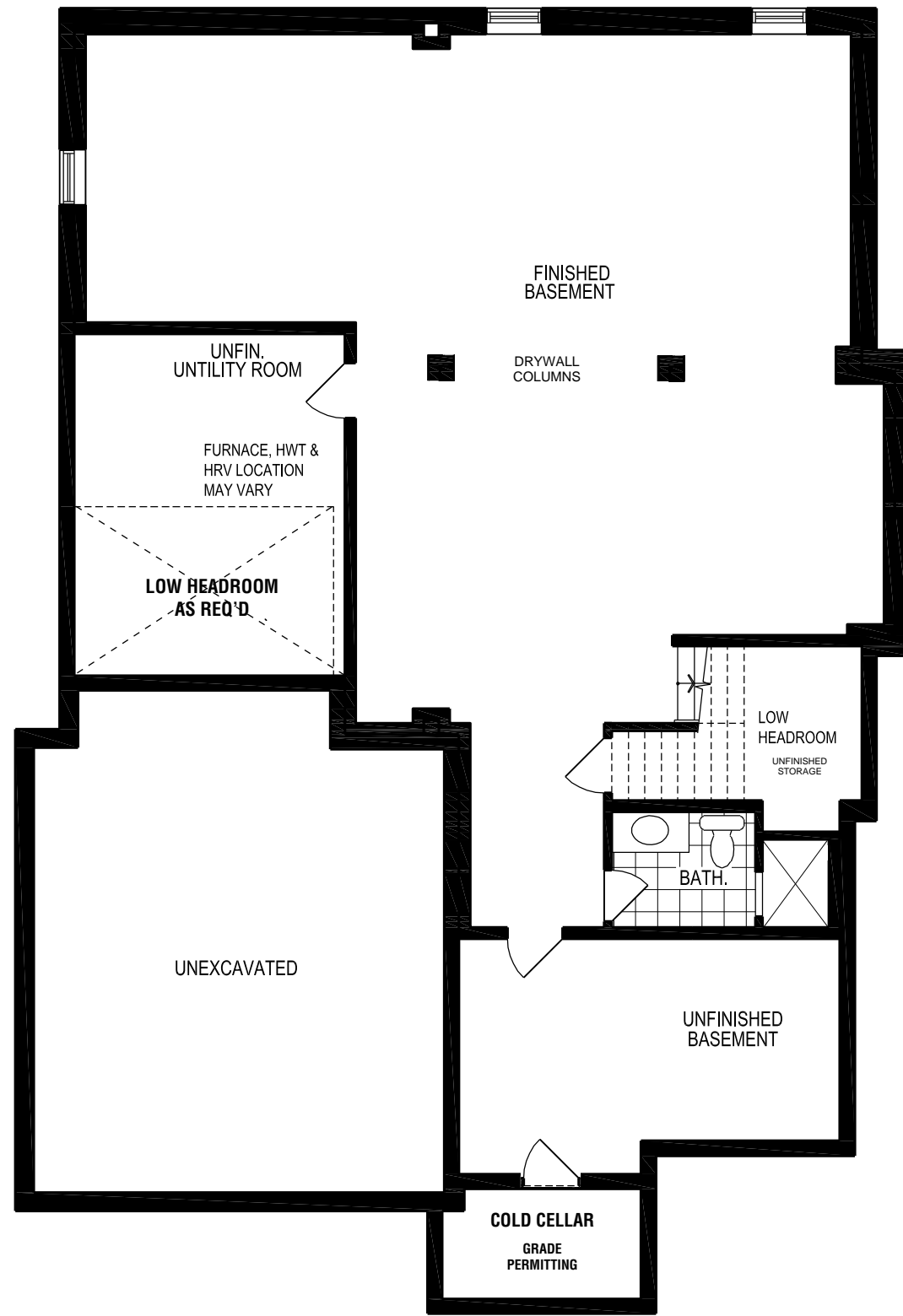
BASEMENT PLAN
